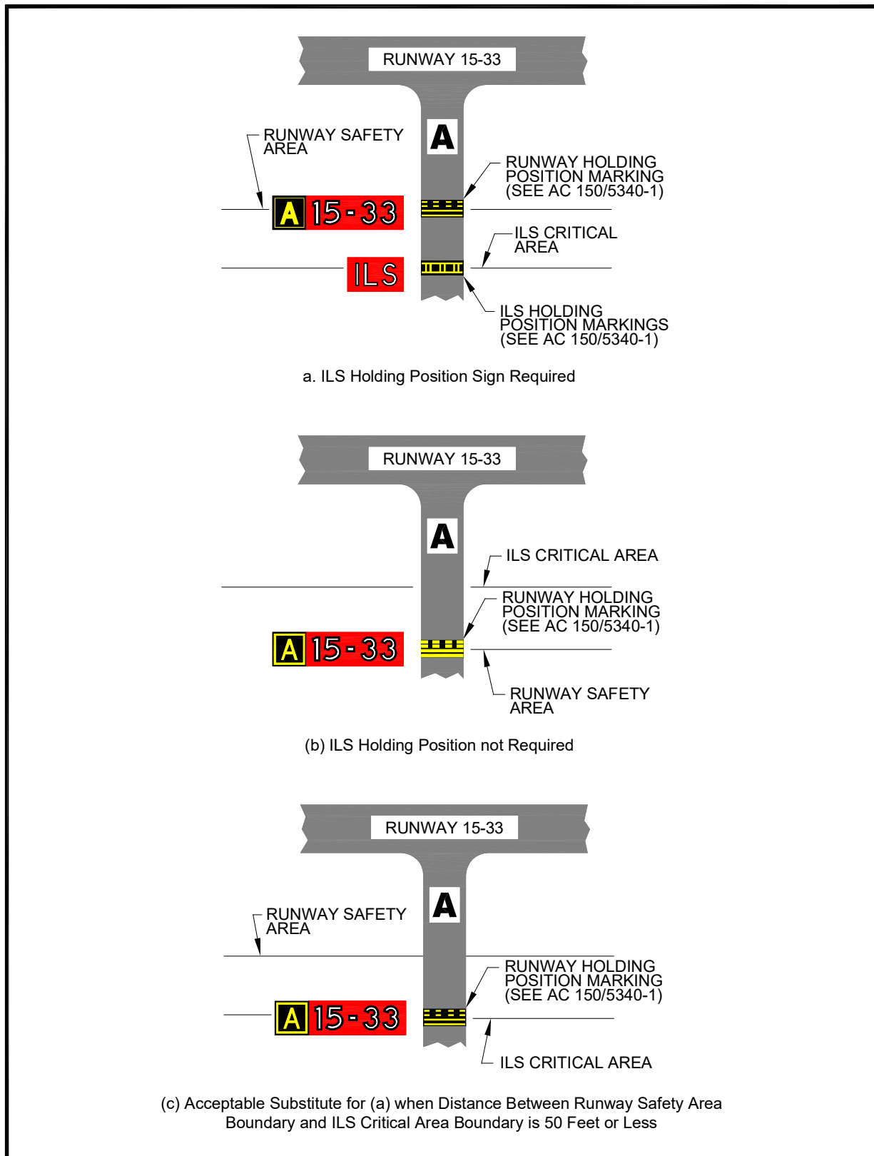
Figure 1-9. Sign Applications for ILS Critical Areas.
