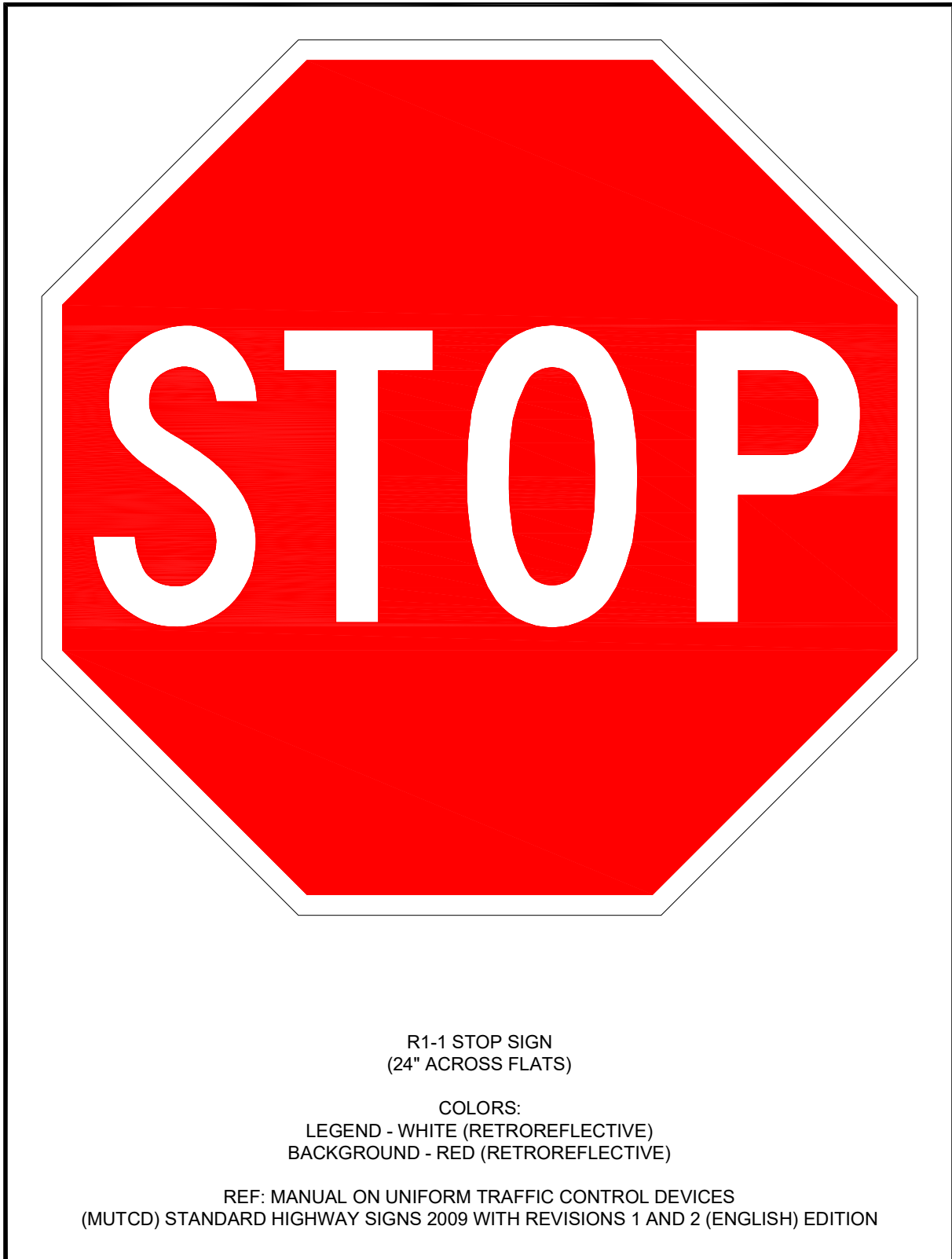
Figure 1-17. STOP Sign.
