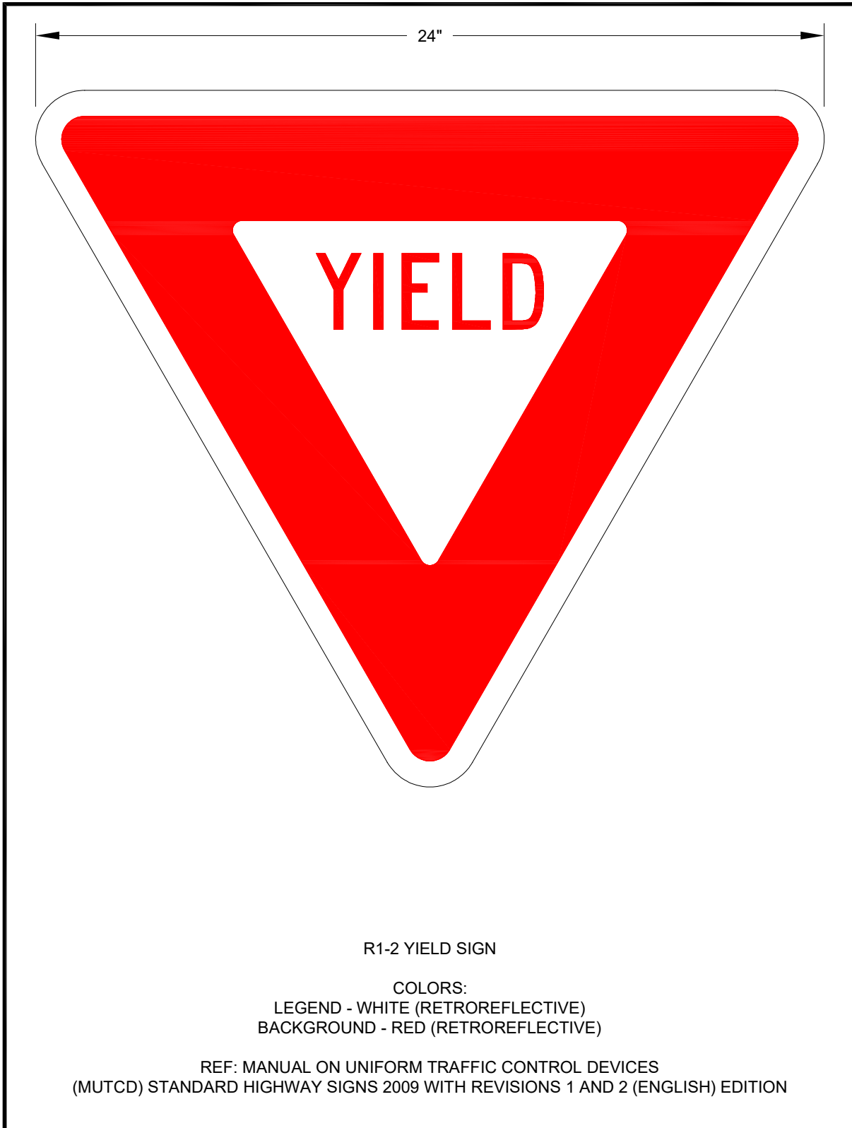
Figure 1-18. YIELD Sign.
